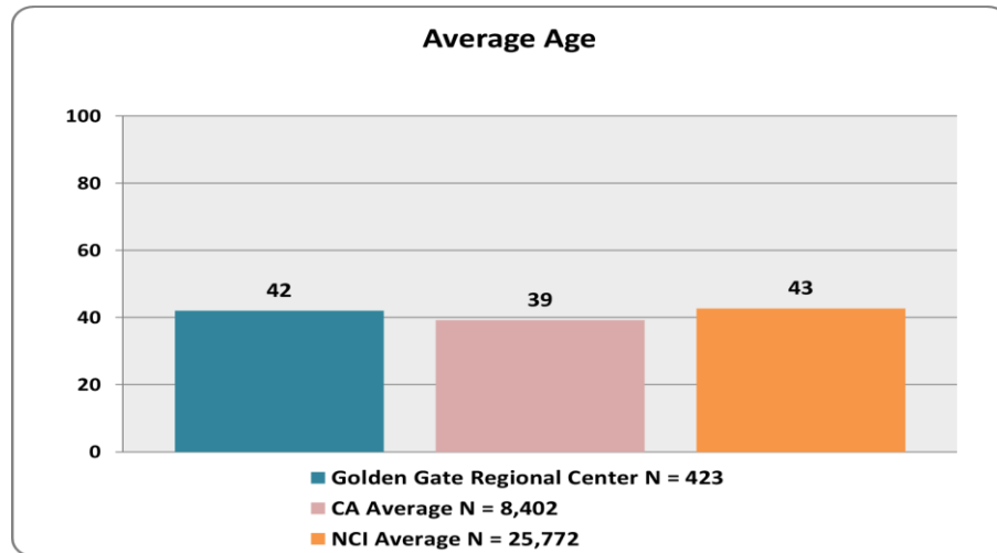
GRAPH 1. AVERAGE AGE
