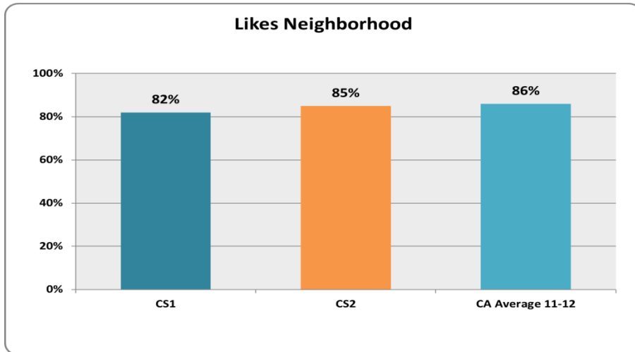
GRAPH 49. LIKES NEIGHBORHOOD
