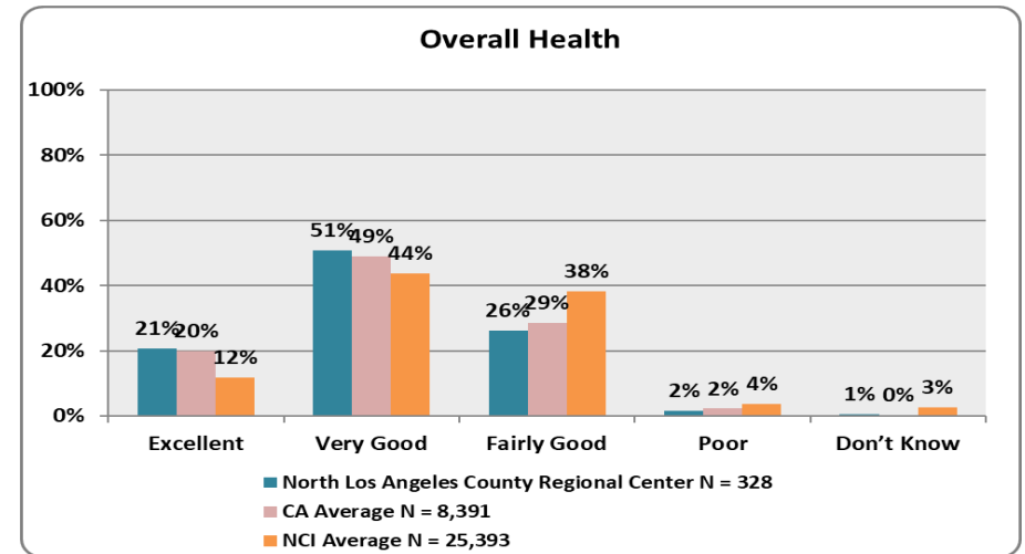
GRAPH 72. OVERALL HEALTH
