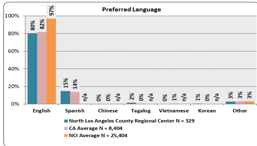
GRAPH 12. PREFERRED LANGUAGE
